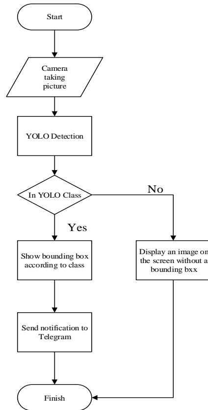
Fig 3. Flowchart of the YOLO v4 Work System
